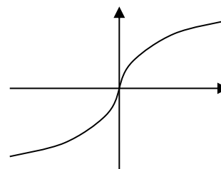
origin symmetry
