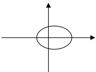
x-axis symmetry
