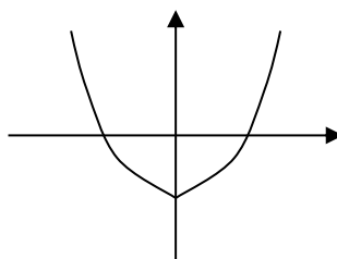
y-axis symmetry
